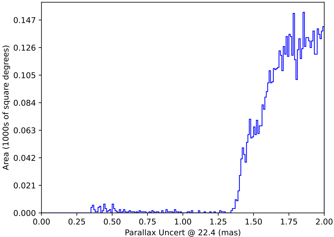
too_elab_r128_d3_gz_v3.4_10yrs : Parallax Uncert @ 22.4
