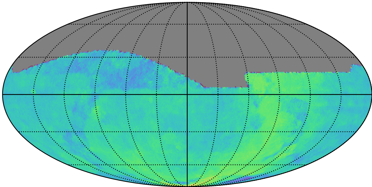
too_elab_r128_d3_gz_v3.4_10yrs : Parallax Coverage @ 22.4
