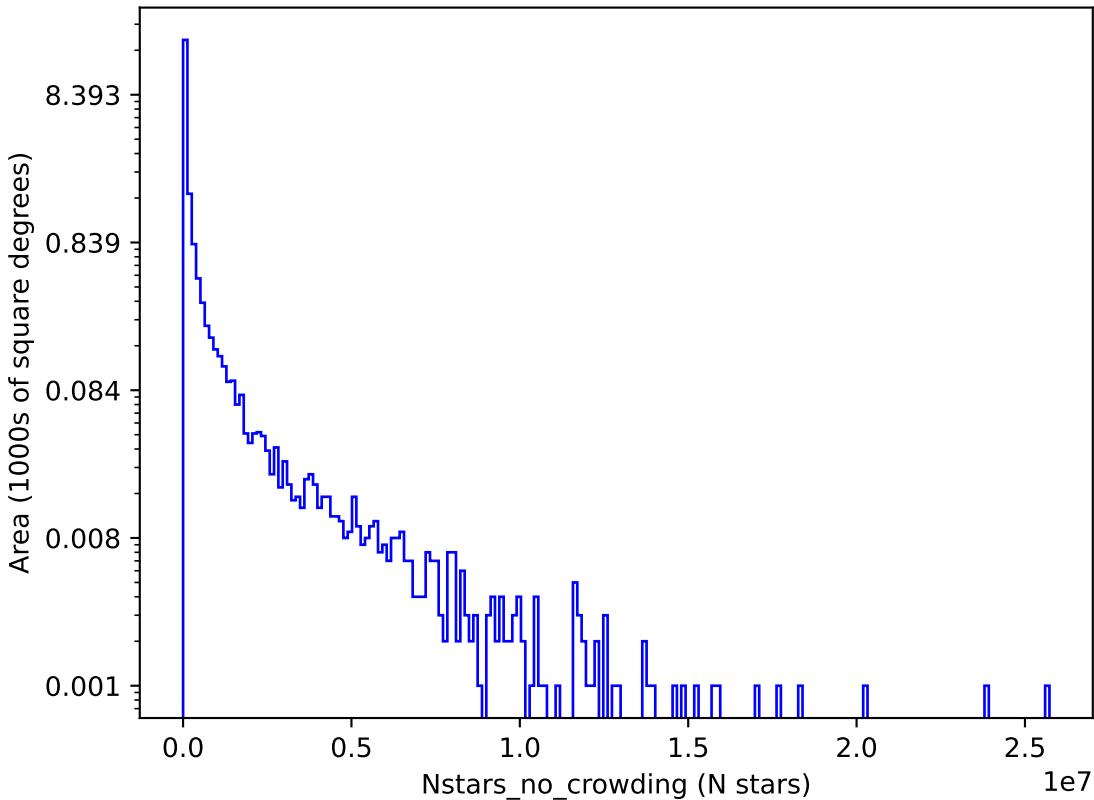
too_elab_r128_d3_gz_v3.4_10yrs y: Nstars_no_crowding
