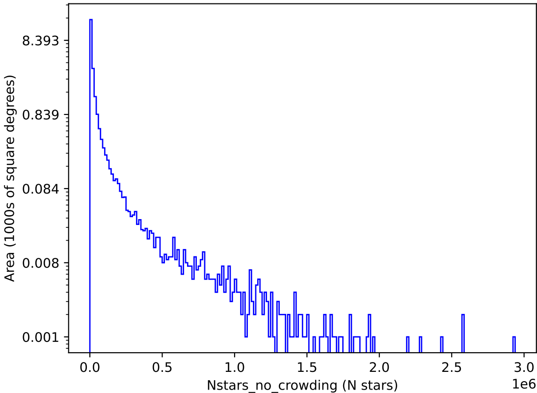
too_elab_r128_d3_gz_v3.4_10yrs u: Nstars_no_crowding
