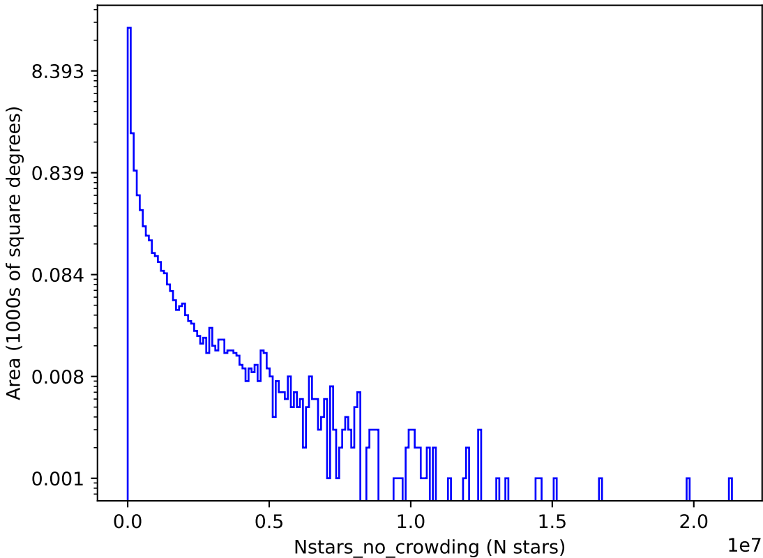
too_elab_r128_d3_gz_v3.4_10yrs r: Nstars_no_crowding
