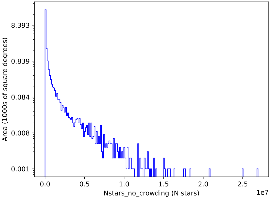
too_elab_r128_d3_gz_v3.4_10yrs i: Nstars_no_crowding
