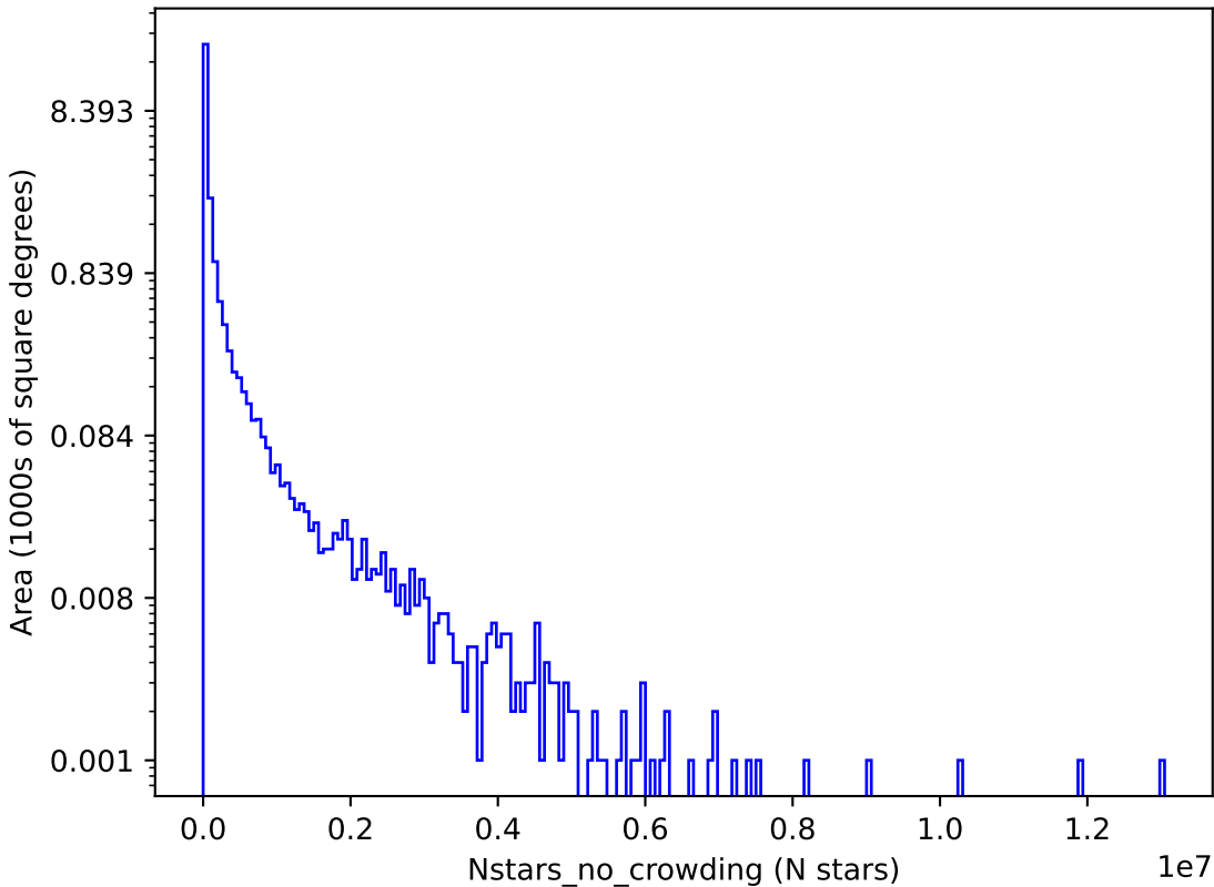
too_elab_r128_d3_gz_v3.4_10yrs g: Nstars_no_crowding
