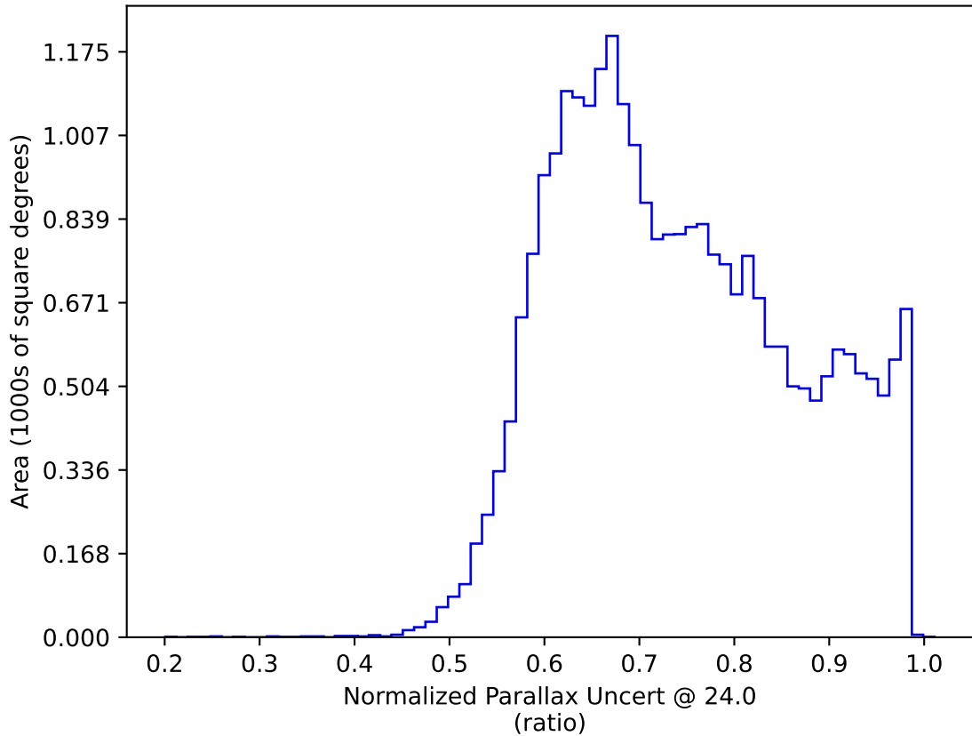
too_elab_r128_d3_gz_v3.4_10yrs : Normalized Parallax Uncert @ 24.0
