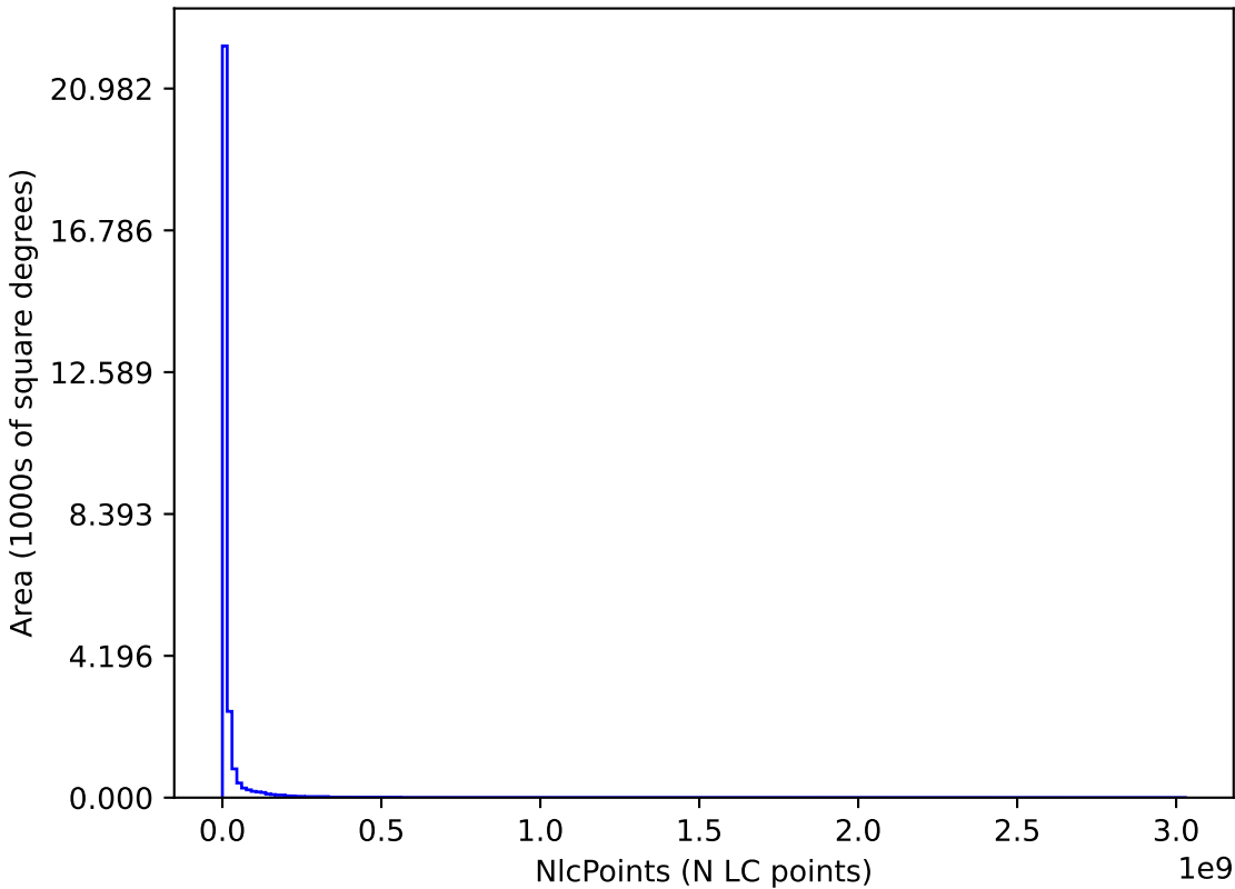
too_elab_r128_d3_gz_v3.4_10yrs : NlcPoints
