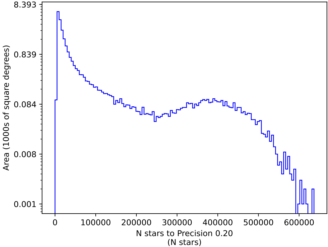
too_elab_r128_d3_gz_v3.4_10yrs z: N stars to Precision 0.20
