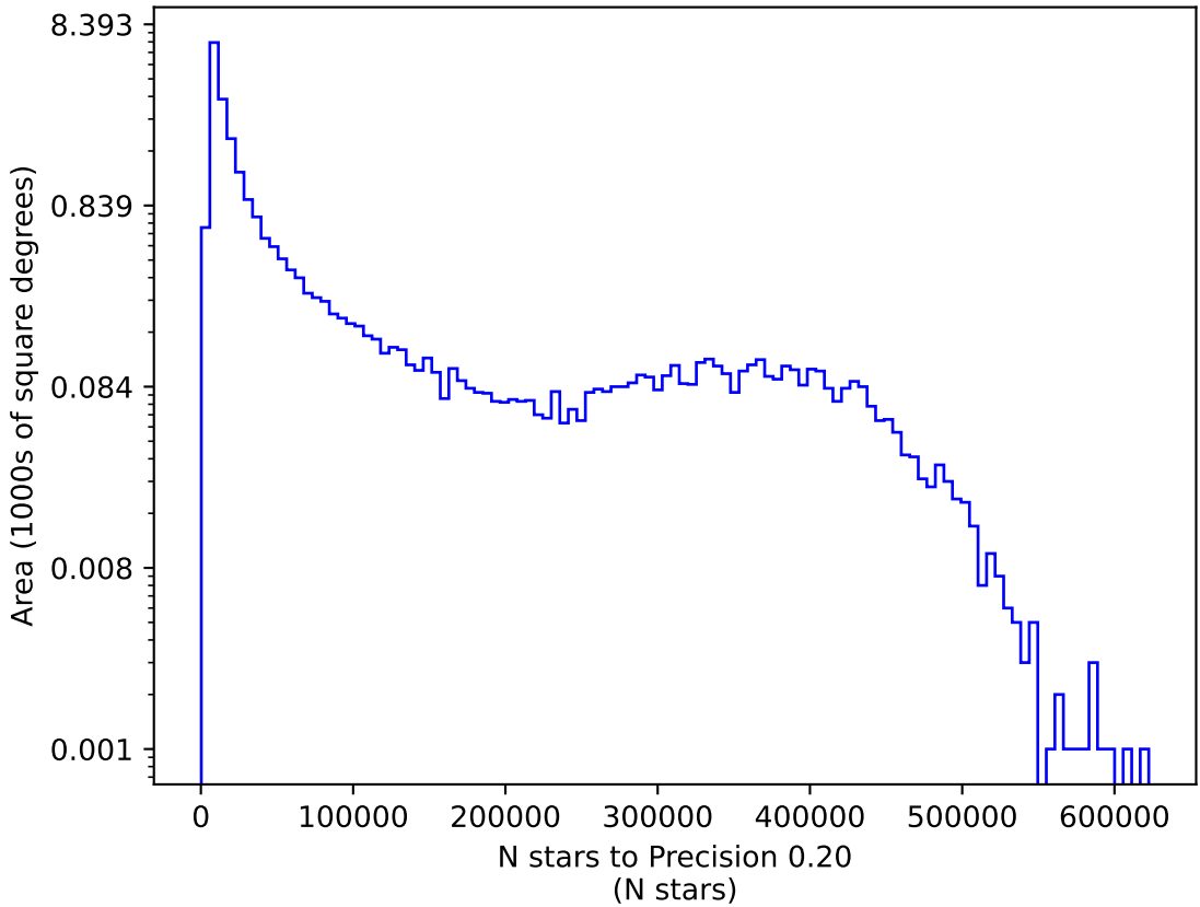
too_elab_r128_d3_gz_v3.4_10yrs y: N stars to Precision 0.20
