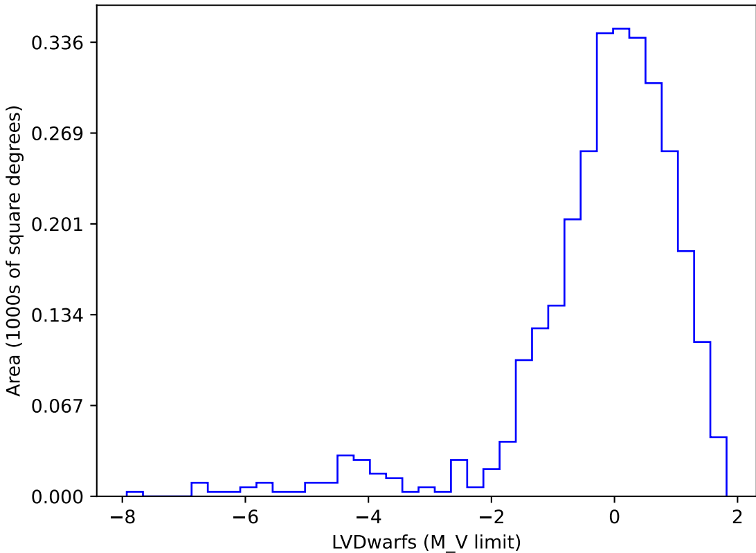
too_elab_r128_d3_gz_v3.4_10yrs gi SCP: LVDwarfs
