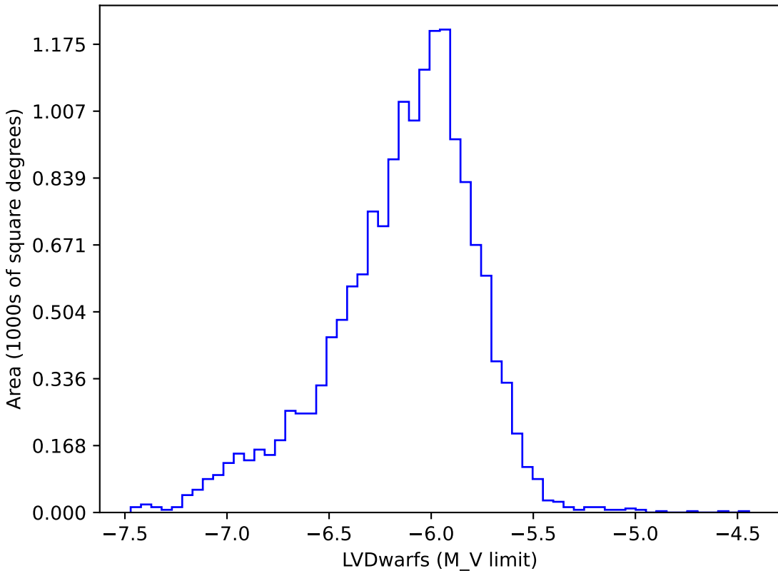
too_elab_r128_d3_gz_v3.4_10yrs gi: LVDwarfs
