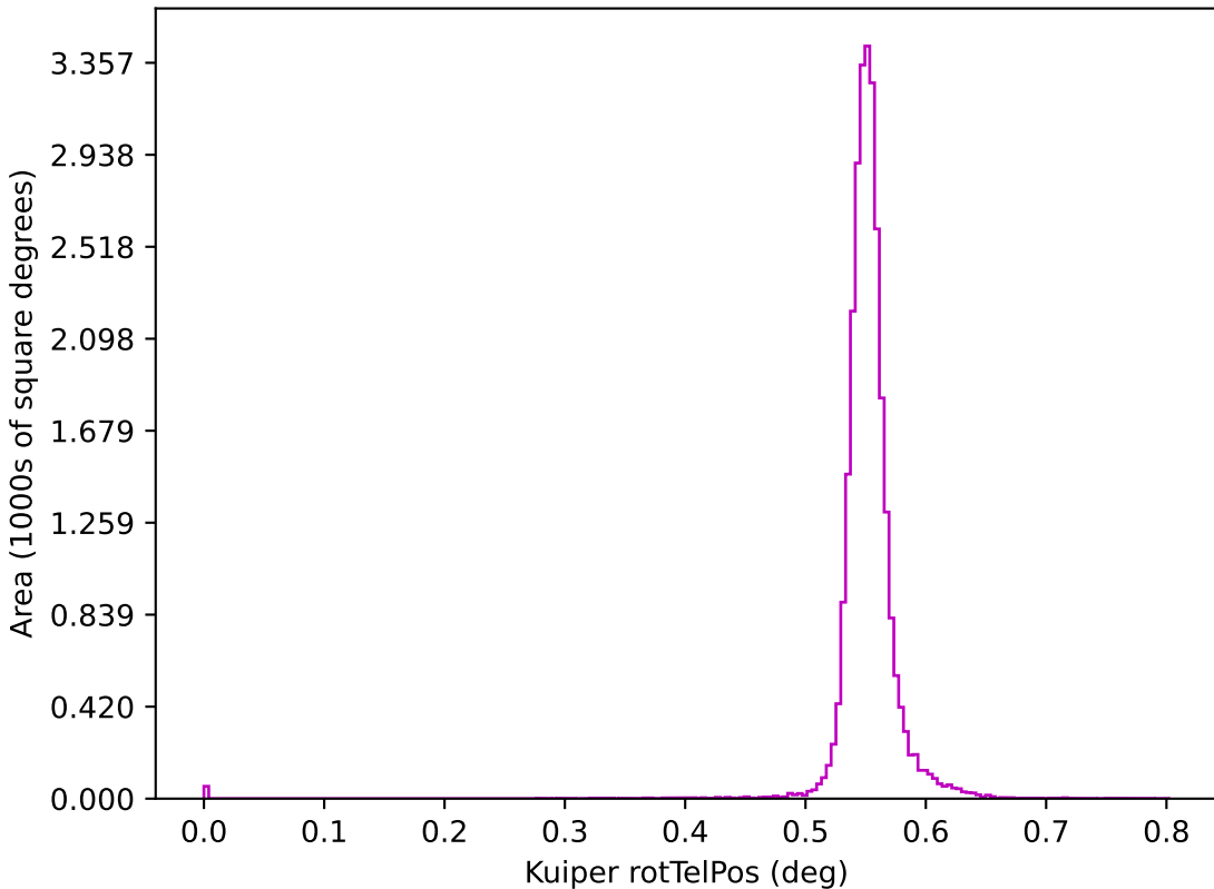
too_elab_r128_d3_gz_v3.4_10yrs z: Kuiper rotTelPos
