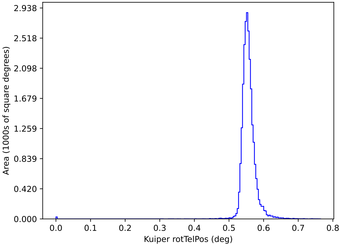
too_elab_r128_d3_gz_v3.4_10yrs y: Kuiper rotTelPos
