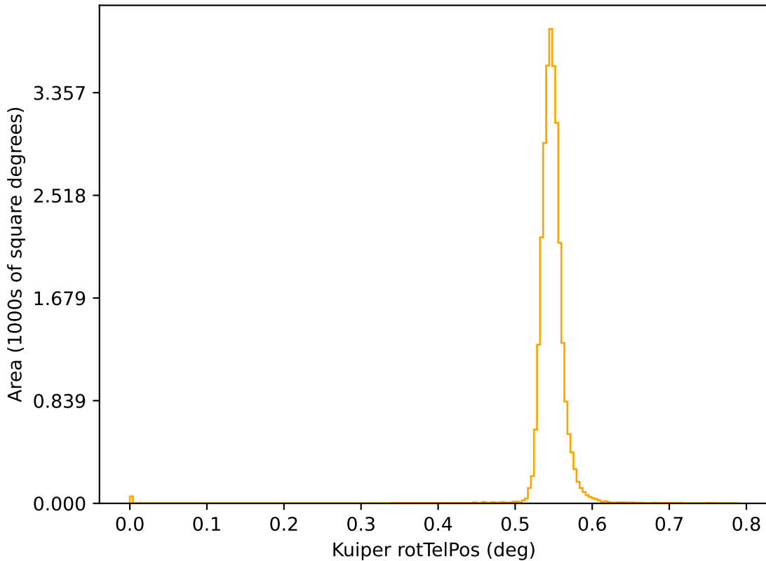
too_elab_r128_d3_gz_v3.4_10yrs r: Kuiper rotTelPos
