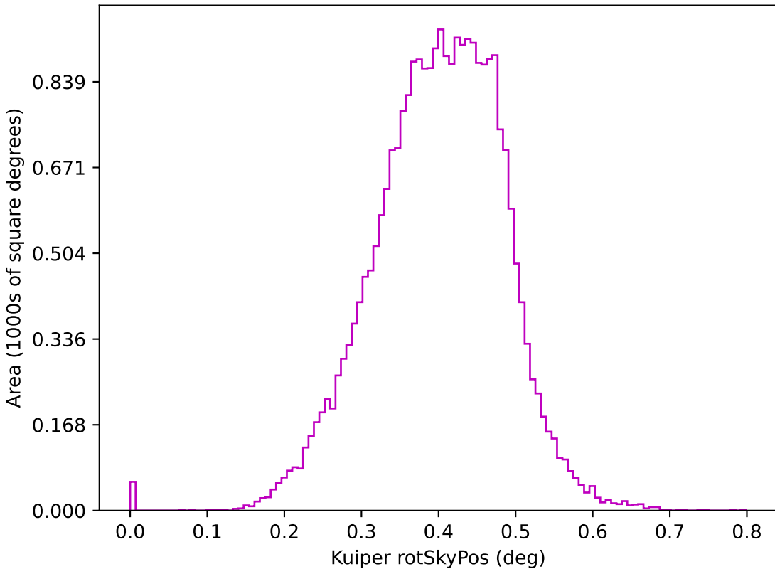
too_elab_r128_d3_gz_v3.4_10yrs z: Kuiper rotSkyPos
