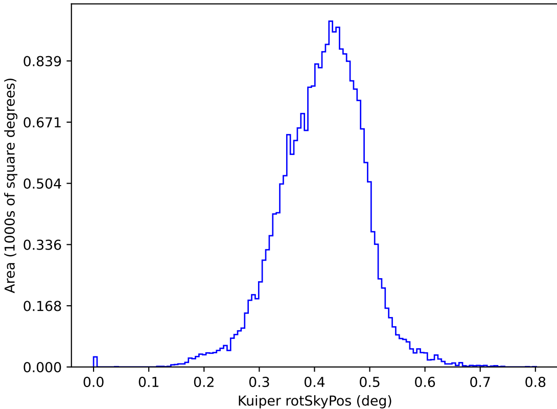
too_elab_r128_d3_gz_v3.4_10yrs y: Kuiper rotSkyPos
