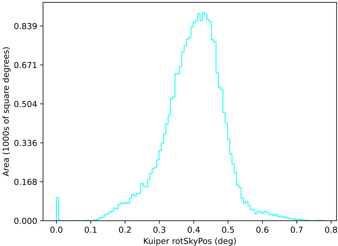
too_elab_r128_d3_gz_v3.4_10yrs u: Kuiper rotSkyPos
