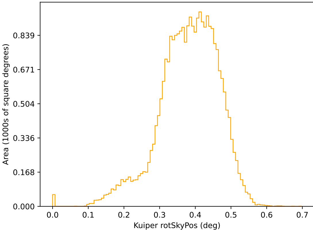
too_elab_r128_d3_gz_v3.4_10yrs r: Kuiper rotSkyPos
