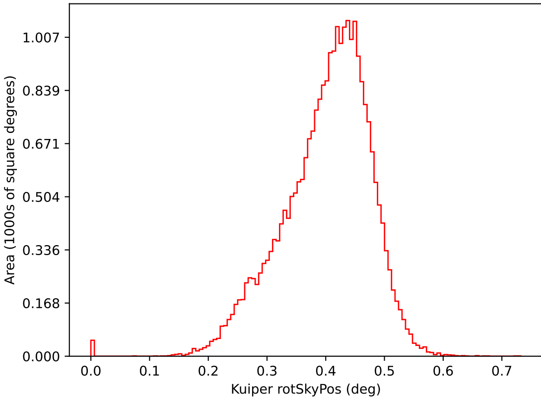
too_elab_r128_d3_gz_v3.4_10yrs i: Kuiper rotSkyPos
