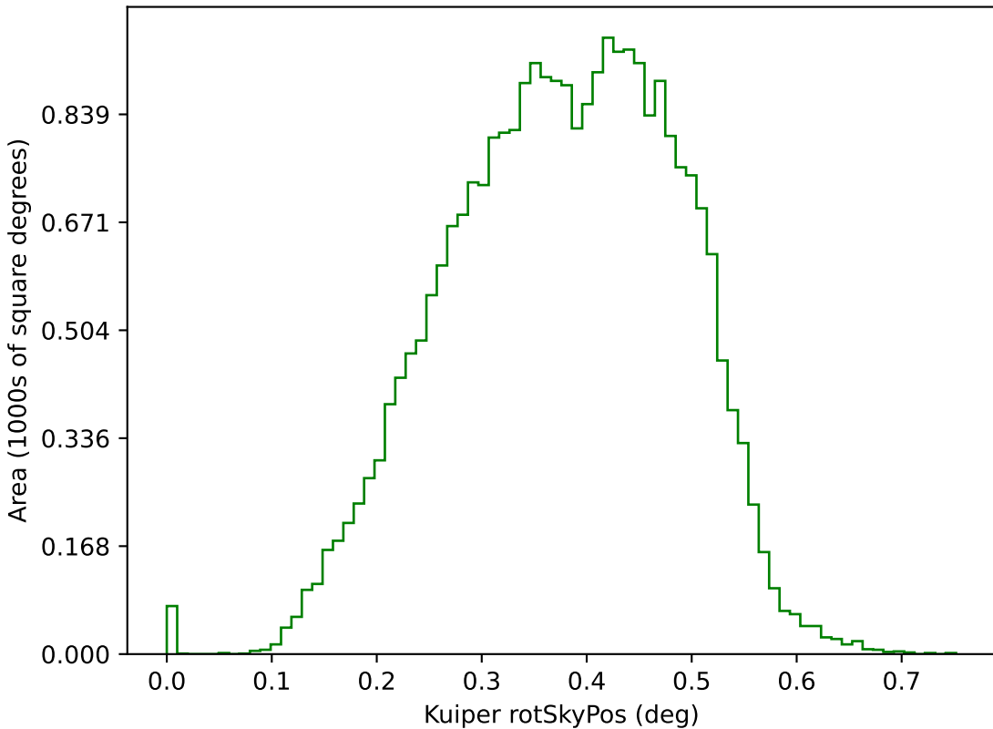
too_elab_r128_d3_gz_v3.4_10yrs g: Kuiper rotSkyPos
