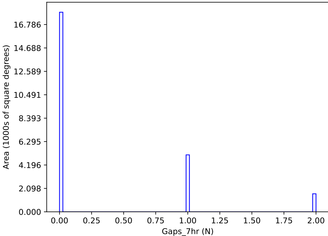
too_elab_r128_d3_gz_v3.4_10yrs y band: Gaps_7hr
