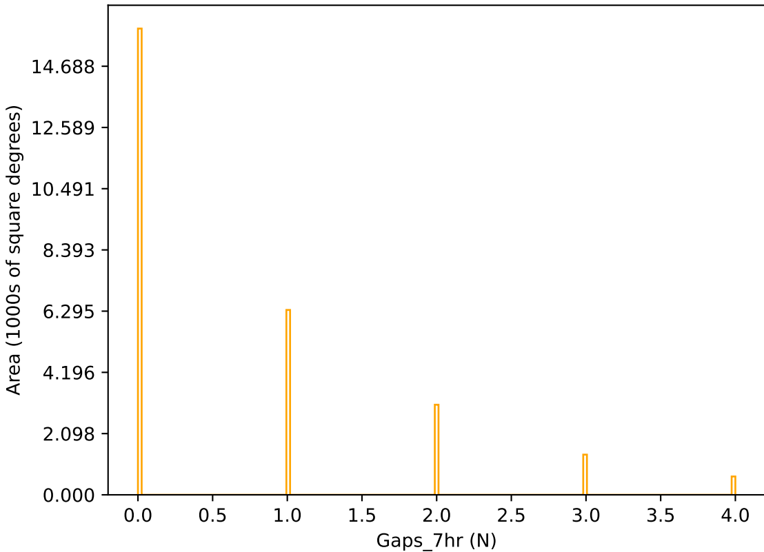
too_elab_r128_d3_gz_v3.4_10yrs r band: Gaps_7hr
