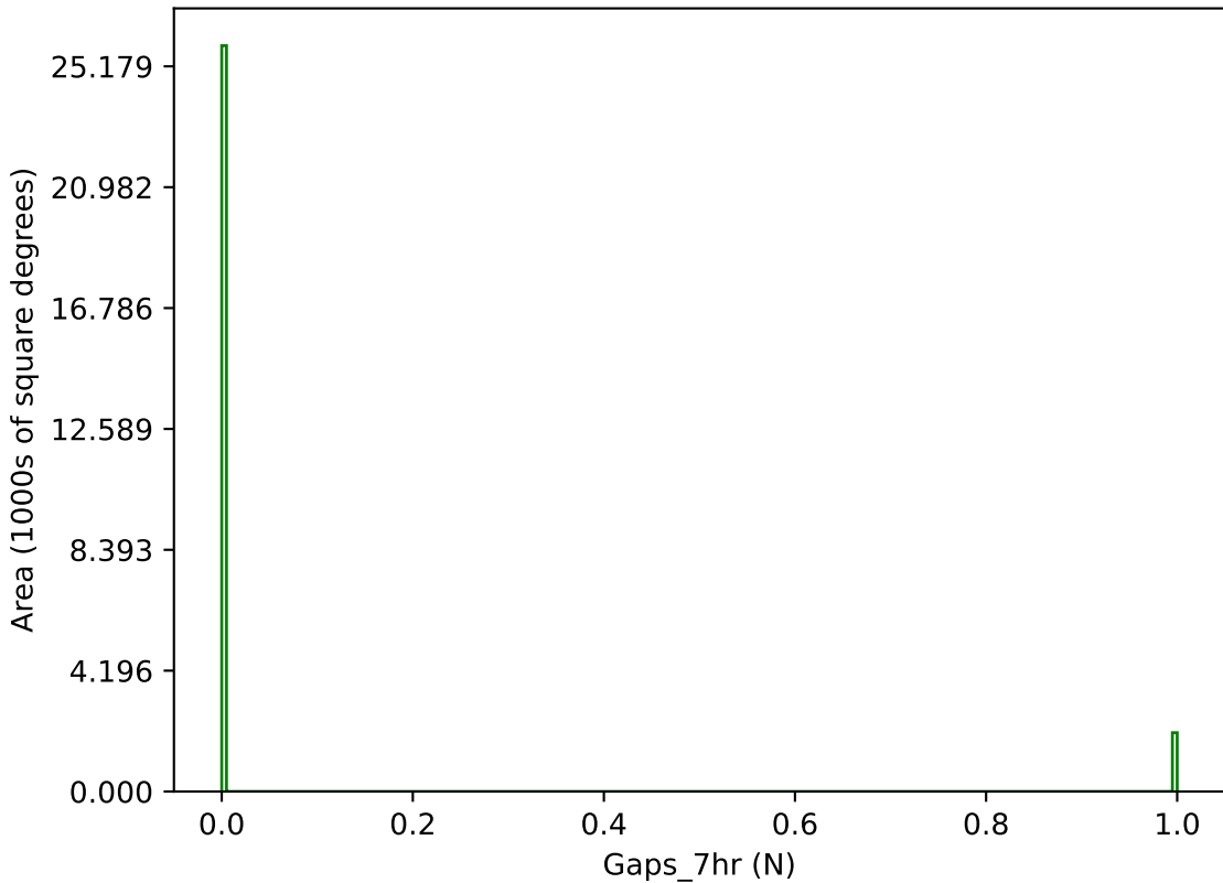
too_elab_r128_d3_gz_v3.4_10yrs g band: Gaps_7hr
