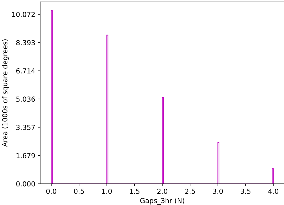
too_elab_r128_d3_gz_v3.4_10yrs z band: Gaps_3hr
