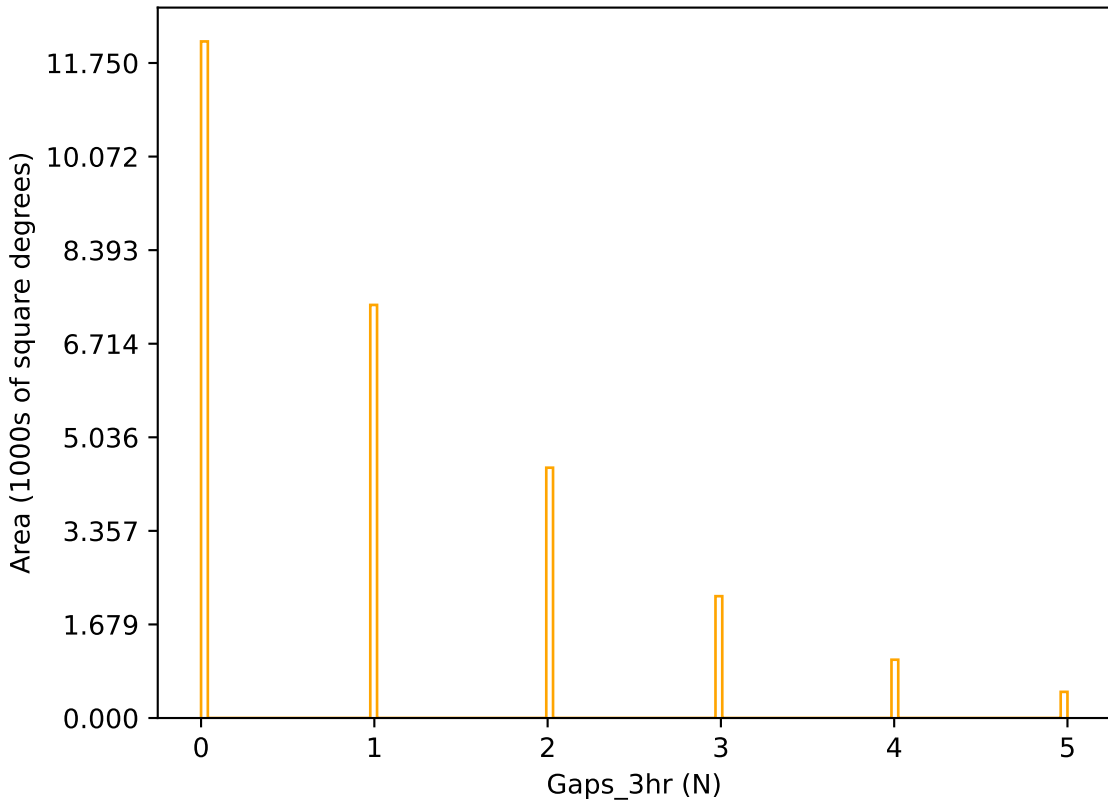
too_elab_r128_d3_gz_v3.4_10yrs r band: Gaps_3hr
