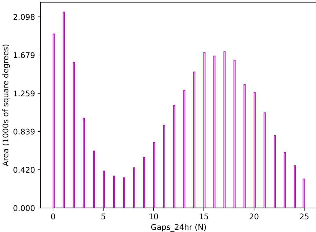
too_elab_r128_d3_gz_v3.4_10yrs z band: Gaps_24hr
