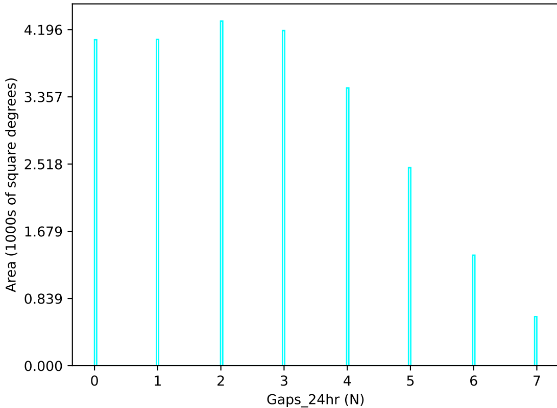
too_elab_r128_d3_gz_v3.4_10yrs u band: Gaps_24hr
