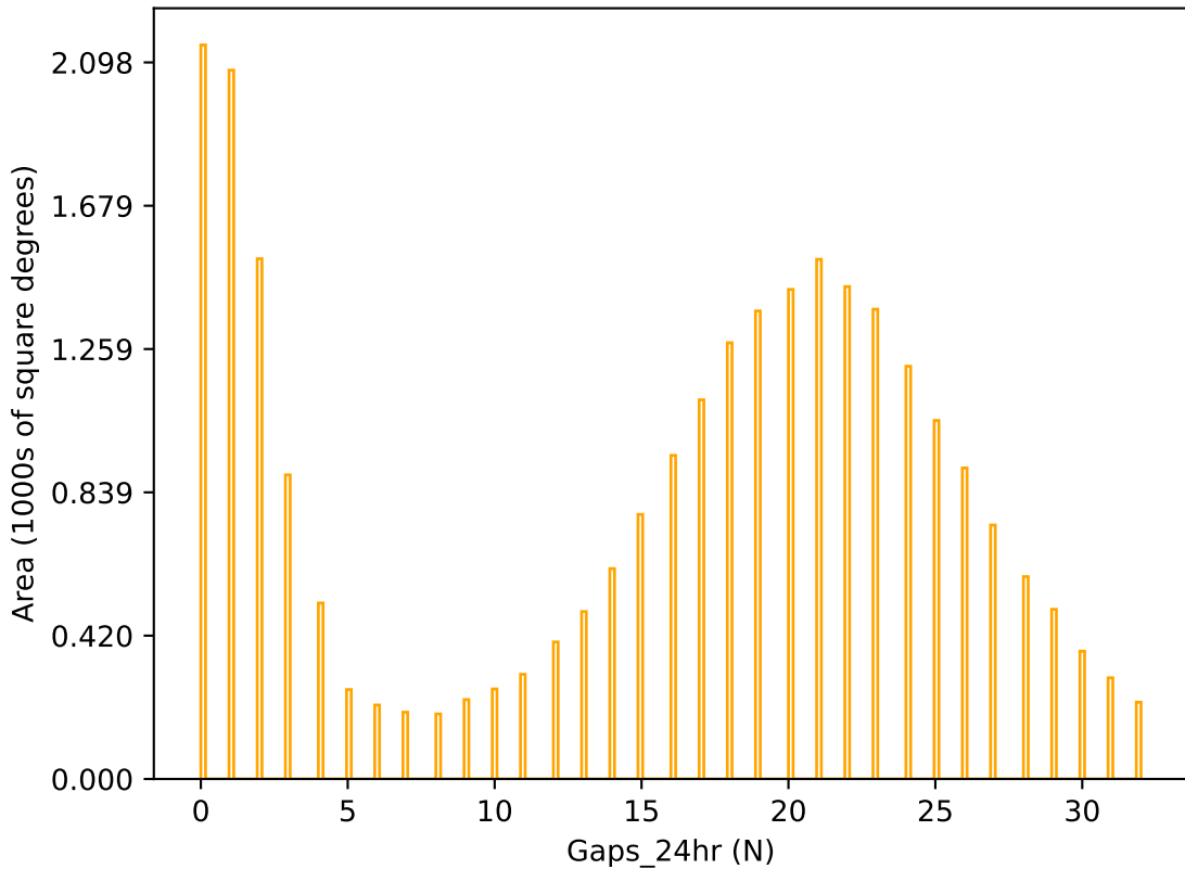
too_elab_r128_d3_gz_v3.4_10yrs r band: Gaps_24hr
