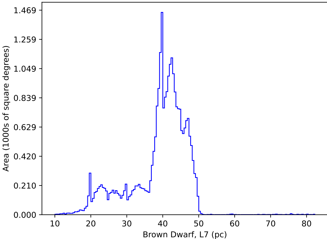
too_elab_r128_d3_gz_v3.4_10yrs : Brown Dwarf, L7
