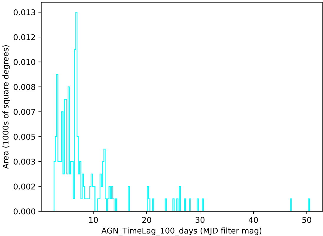
too_elab_r128_d3_gz_v3.4_10yrs u band: AGN_TimeLag_100_days
