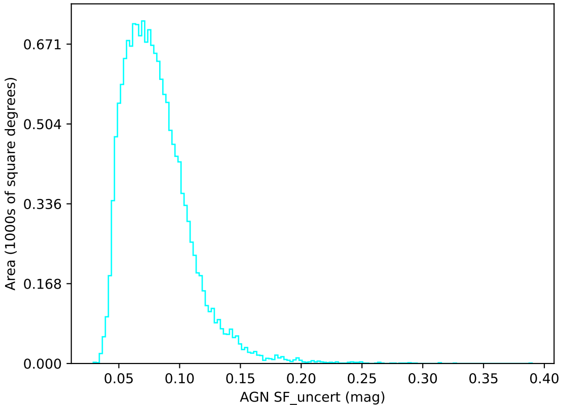
too_elab_r128_d3_gz_v3.4_10yrs u band: AGN SF_uncert
