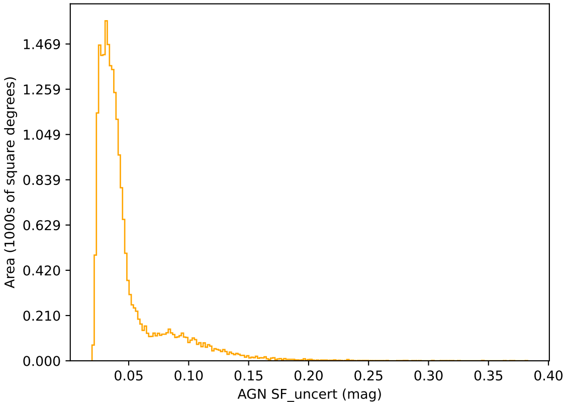
too_elab_r128_d3_gz_v3.4_10yrs r band: AGN SF_uncert
