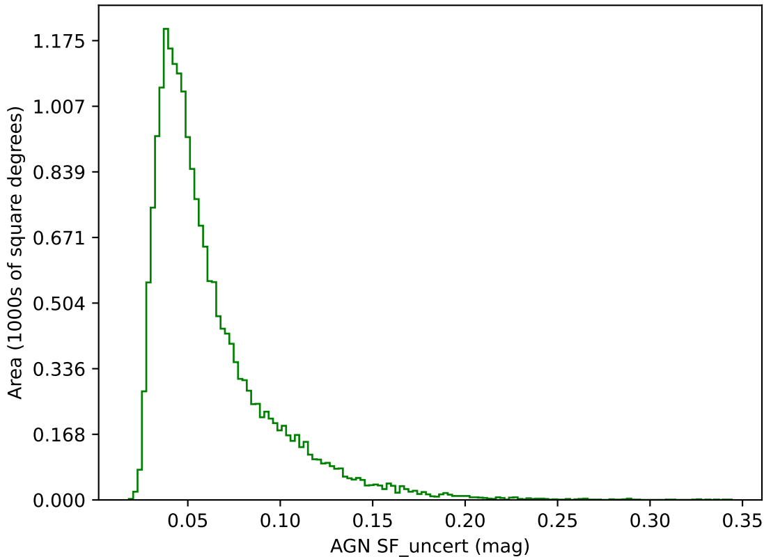
too_elab_r128_d3_gz_v3.4_10yrs g band: AGN SF_uncert
