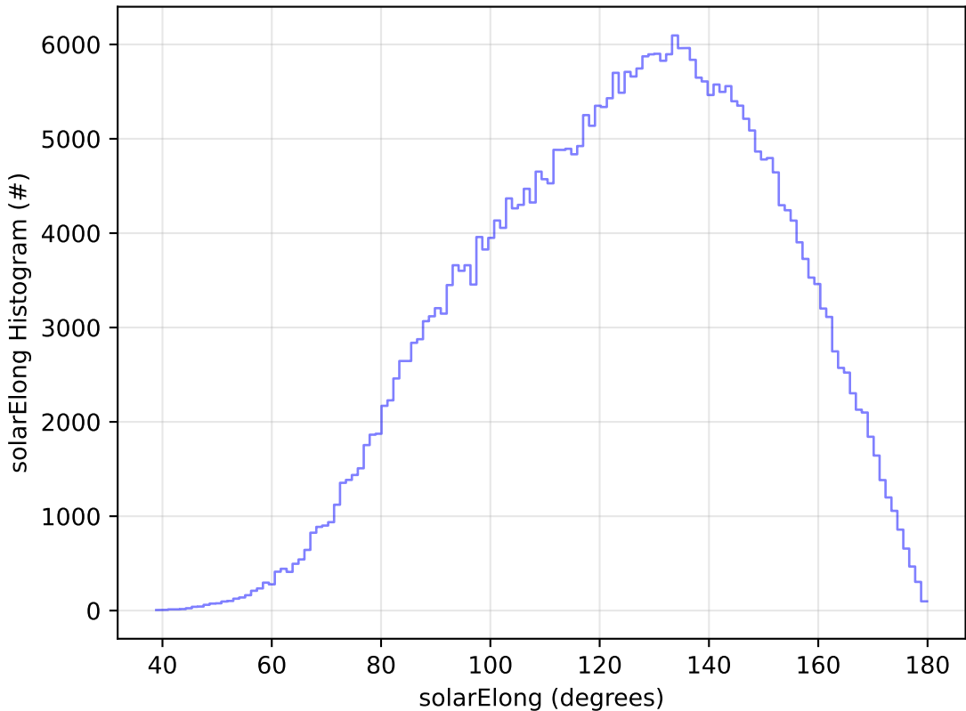
too_elab_r128_d3_gz_v3.4_10yrs WFD y band: solarElong Histogram
