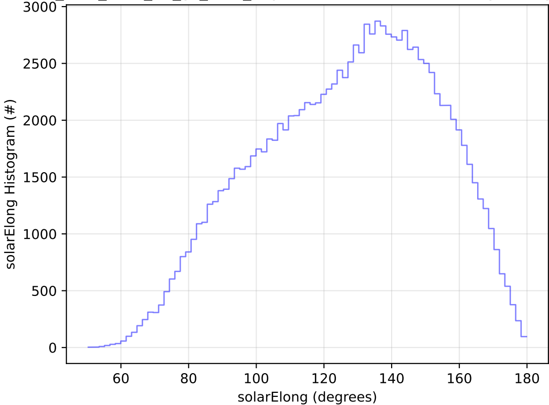
too_elab_r128_d3_gz_v3.4_10yrs WFD u band: solarElong Histogram
