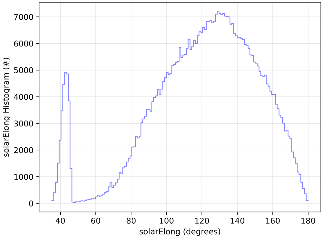
too_elab_r128_d3_gz_v3.4_10yrs WFD i band: solarElong Histogram
