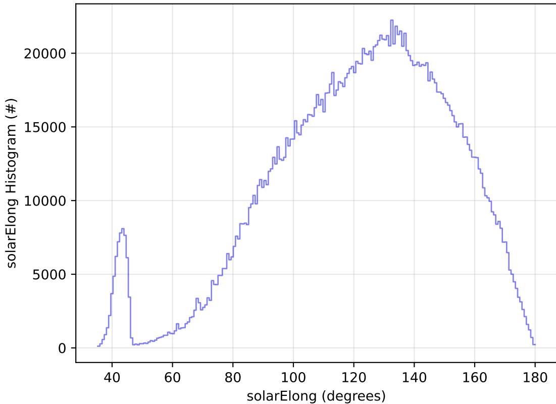
too_elab_r128_d3_gz_v3.4_10yrs WFD all bands: solarElong Histogram
