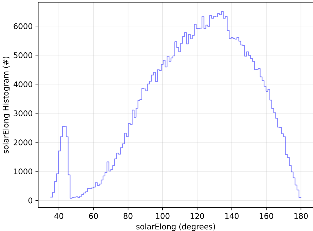
too_elab_r128_d3_gz_v3.4_10yrs All sky z band: solarElong Histogram
