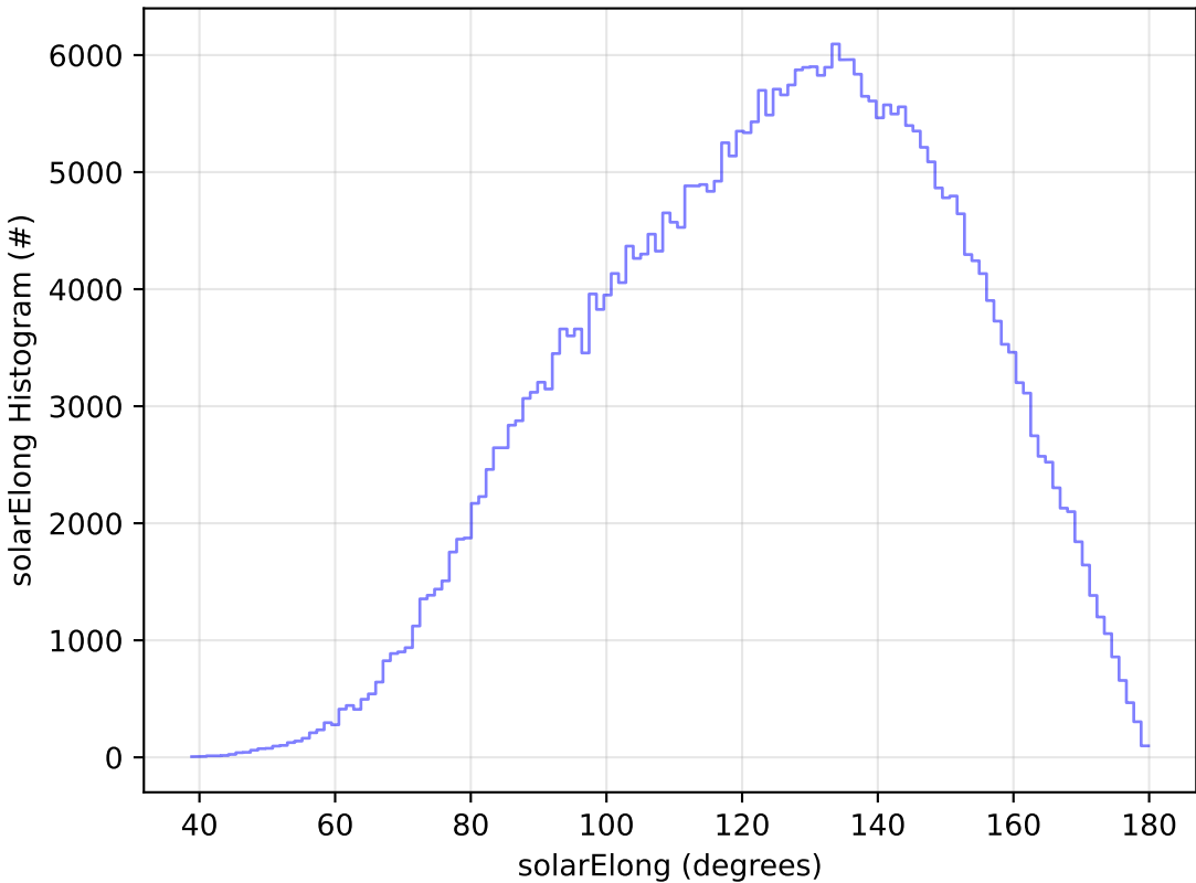
too_elab_r128_d3_gz_v3.4_10yrs All sky y band: solarElong Histogram
