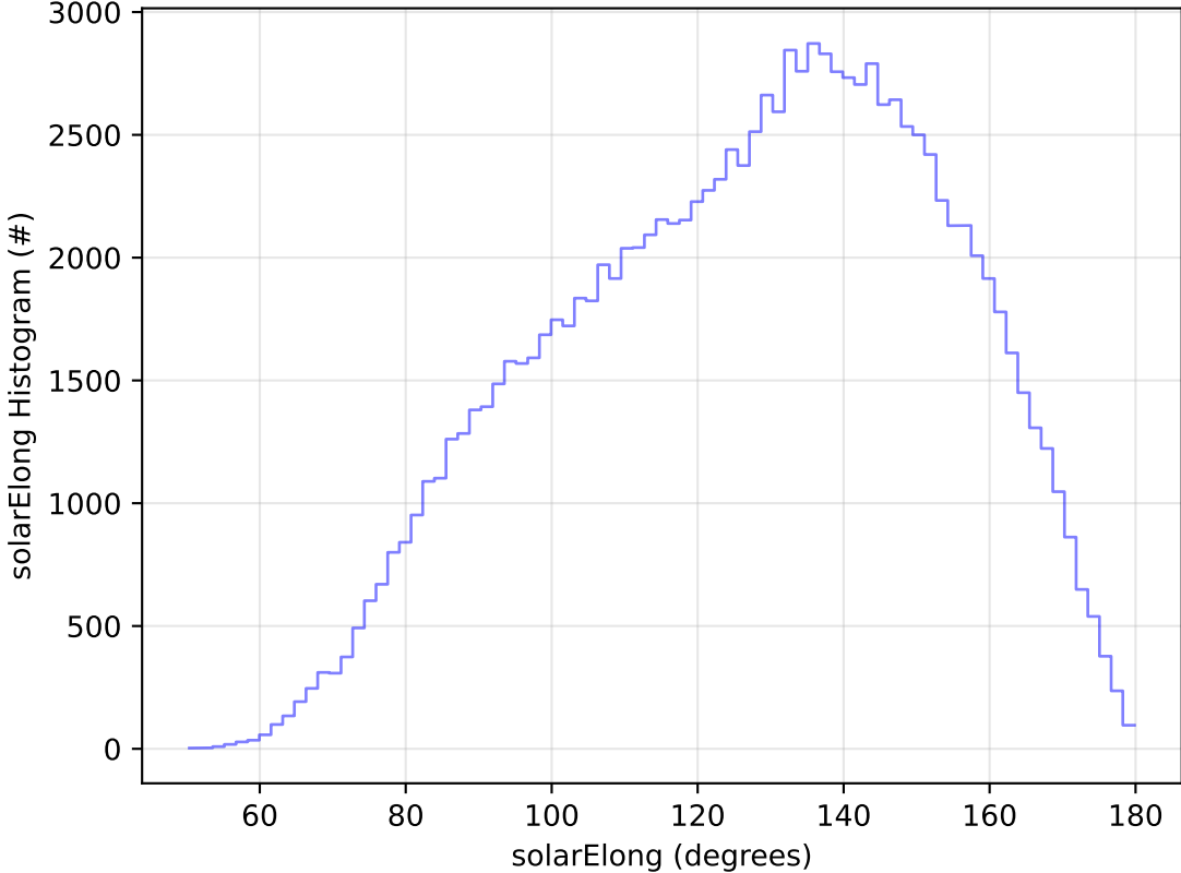
too_elab_r128_d3_gz_v3.4_10yrs All sky u band: solarElong Histogram
