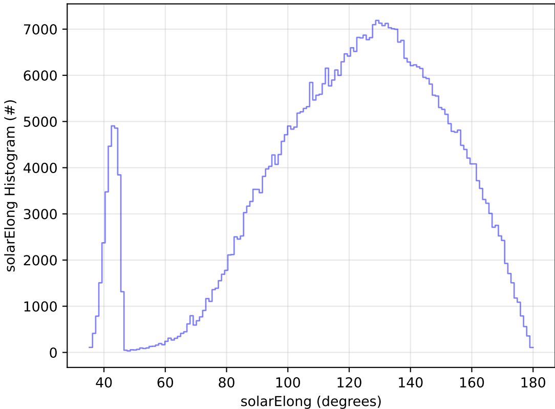
too_elab_r128_d3_gz_v3.4_10yrs All sky i band: solarElong Histogram
