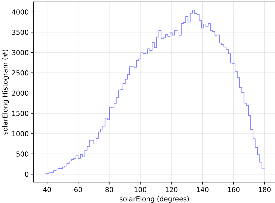
too_elab_r128_d3_gz_v3.4_10yrs All sky g band: solarElong Histogram
