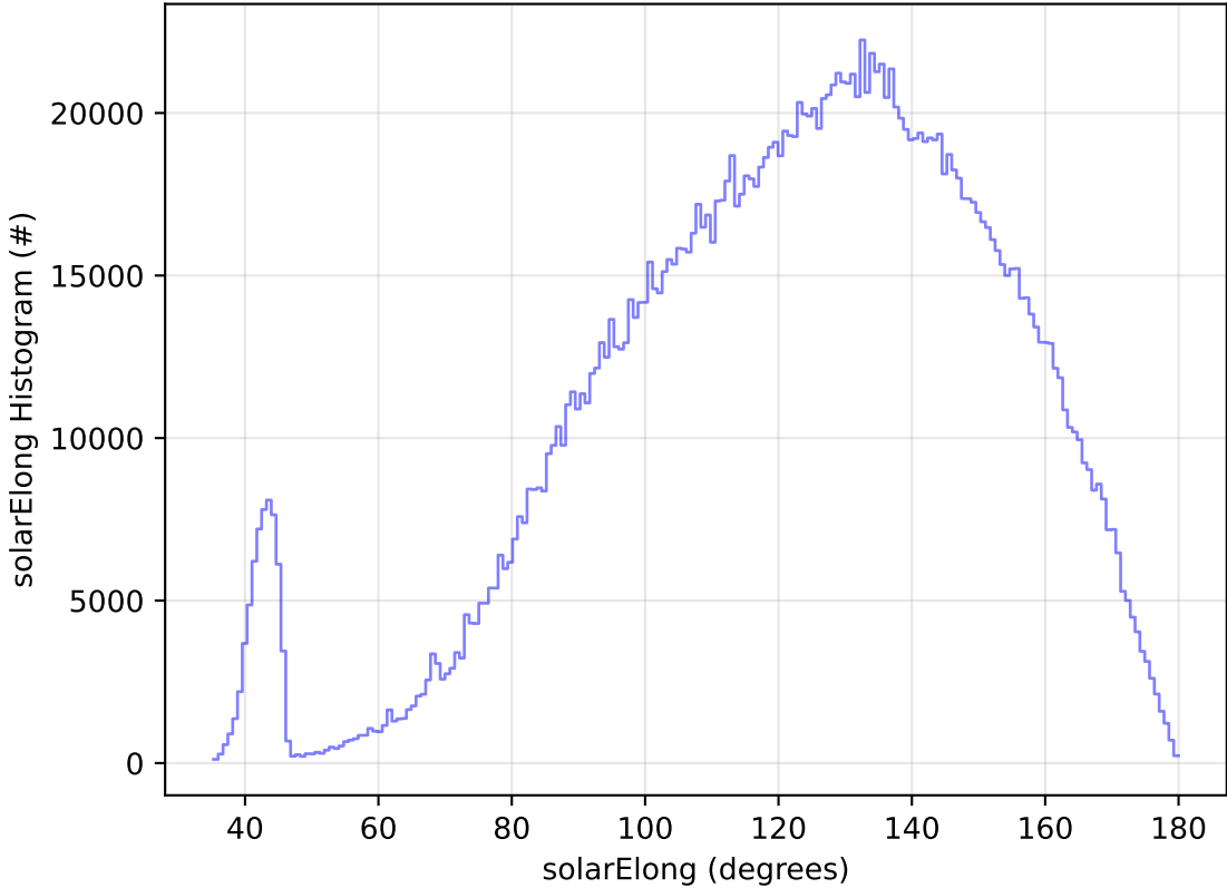
too_elab_r128_d3_gz_v3.4_10yrs All sky all bands: solarElong Histogram
