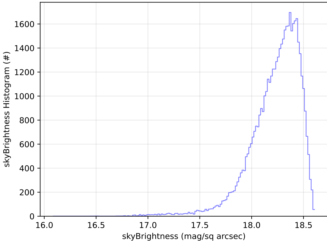
too_elab_r128_d3_gz_v3.4_10yrs Yr 1 y band: skyBrightness Histogram
