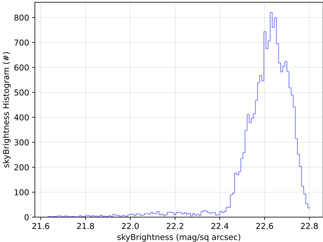
too_elab_r128_d3_gz_v3.4_10yrs Yr 1 u band: skyBrightness Histogram
