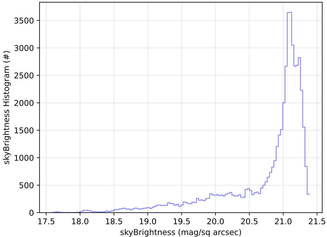
too_elab_r128_d3_gz_v3.4_10yrs Yr 1 r band: skyBrightness Histogram
