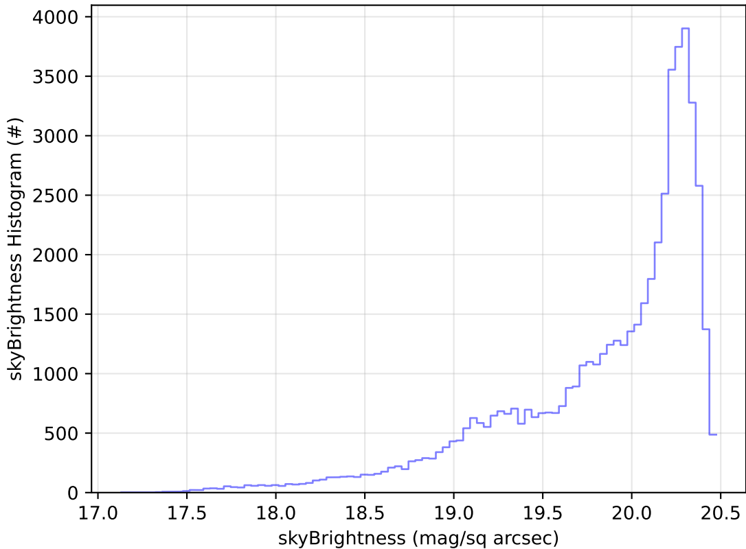
too_elab_r128_d3_gz_v3.4_10yrs Yr 1 i band: skyBrightness Histogram
