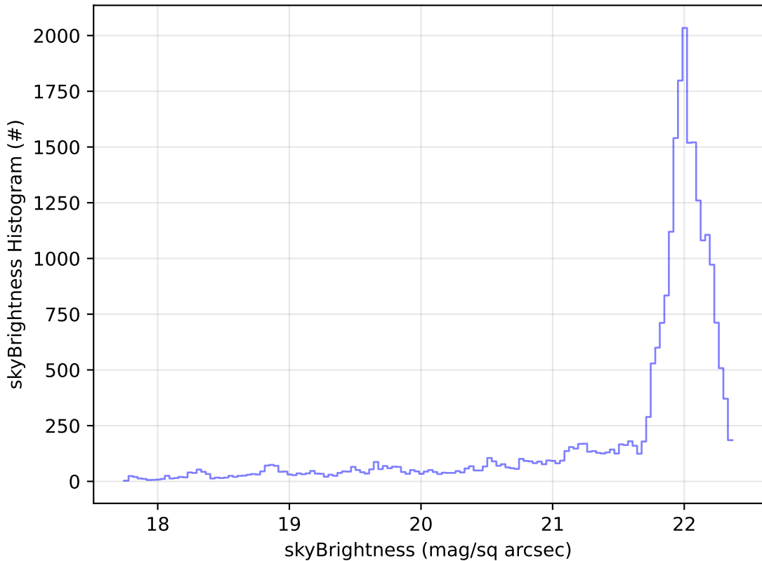
too_elab_r128_d3_gz_v3.4_10yrs Yr 1 g band: skyBrightness Histogram
